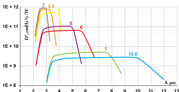
Example of D^* vs Wavelength \lambda for PVI-3TE Series HgCdTe Detectors. Spectral Characteristics of individual detectors may vary from those shown on the chart.
